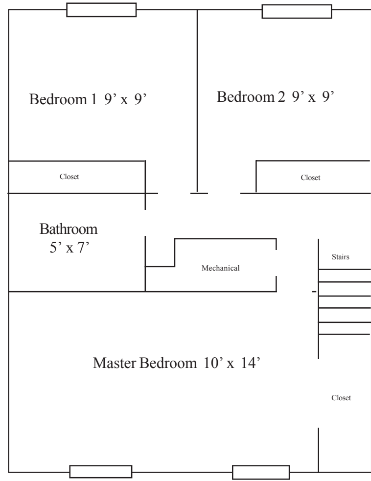
2nd Floor
